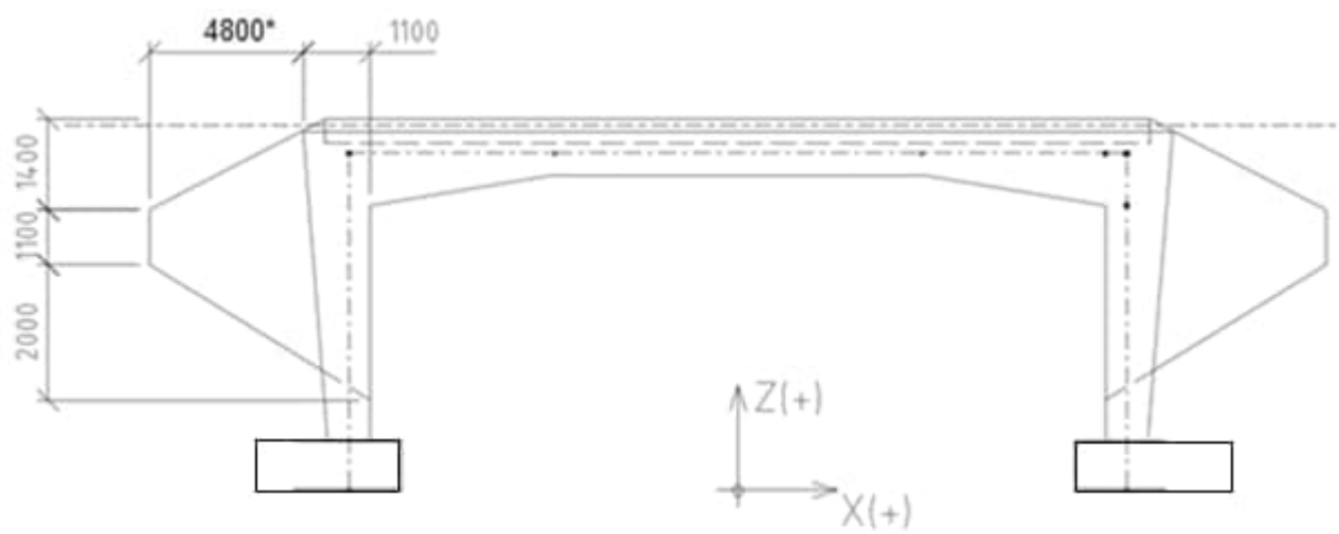
SECTION B-B Wingwalls.
