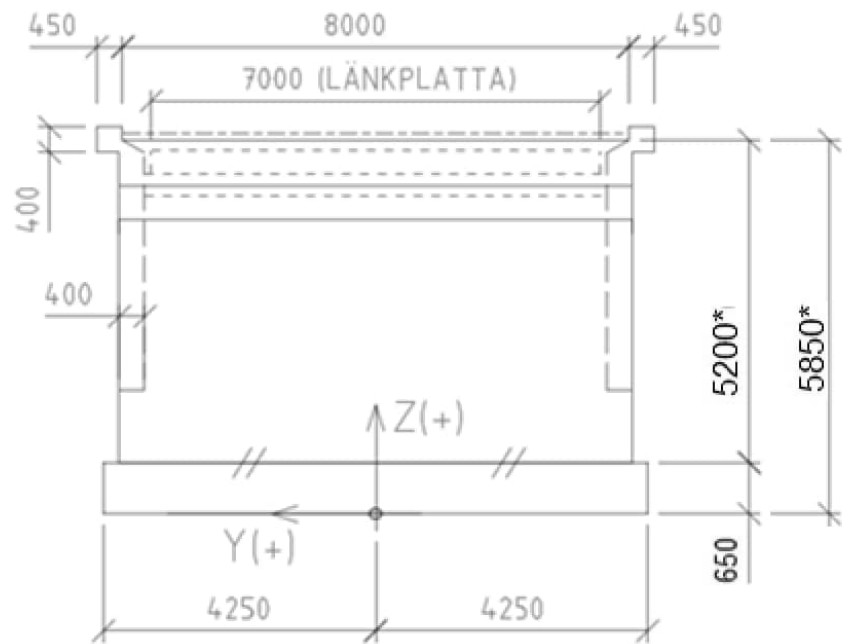
SECTION A-A Transversal direction.
